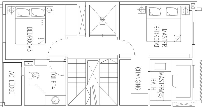
3RD STOREY
