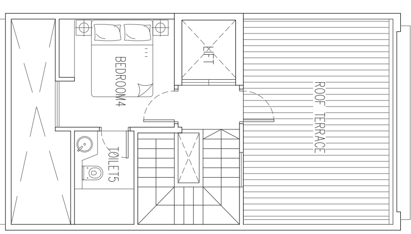
ROOF TERRACE
