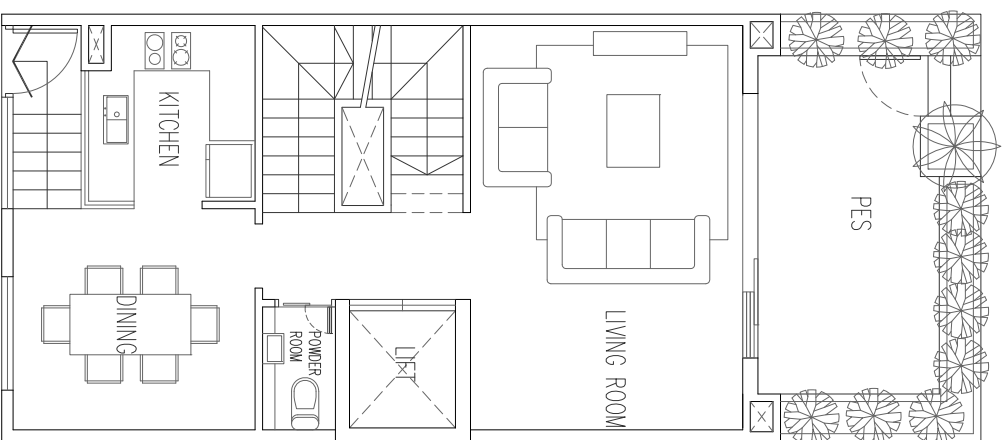
1ST STOREY
