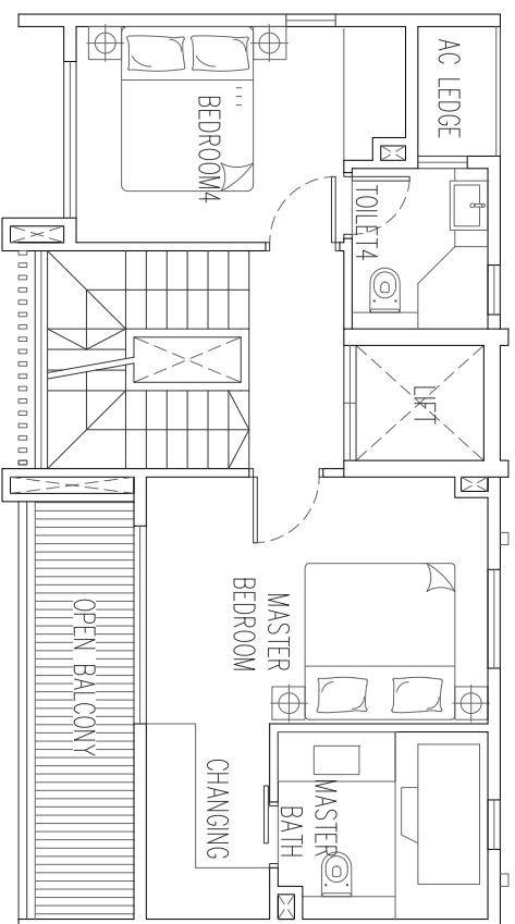
3RD STOREY
