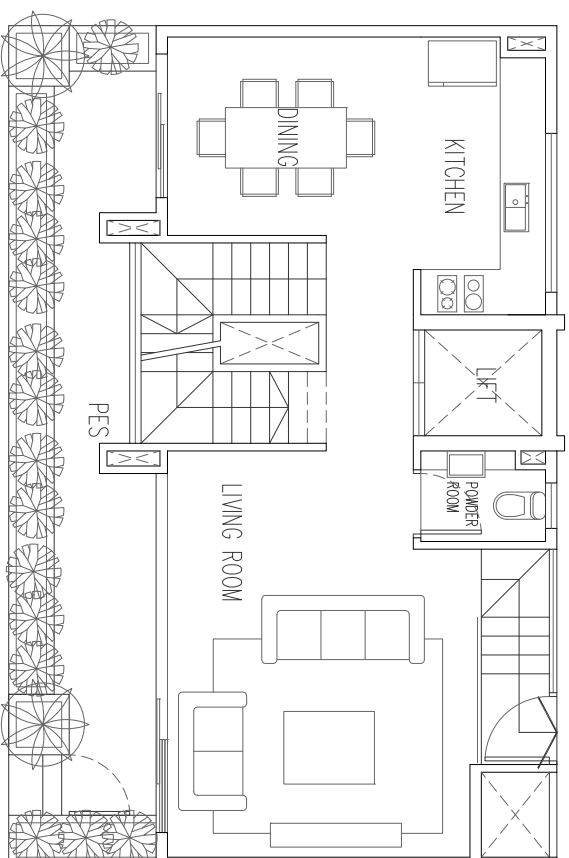
1ST STOREY
