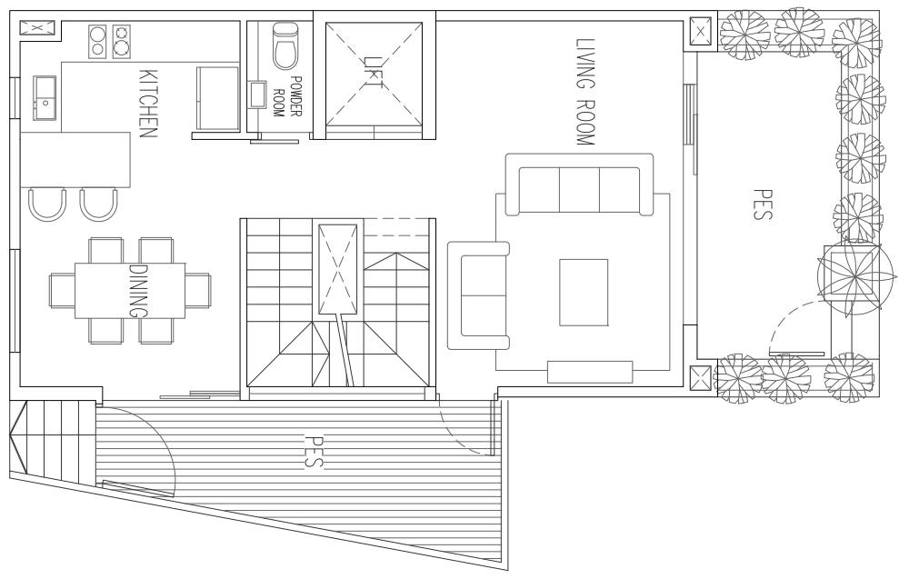
1ST STOREY
