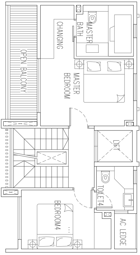
3RD STOREY
