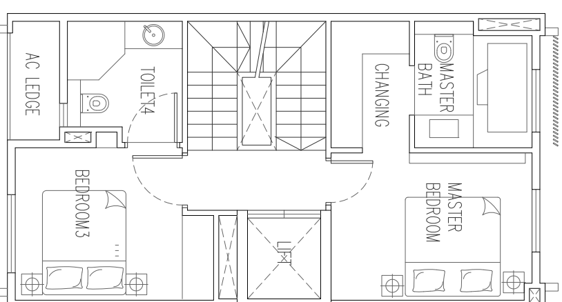
3RD STOREY
