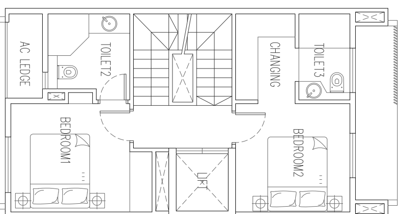
2ND STOREY
