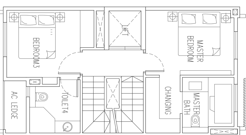
3RD STOREY
