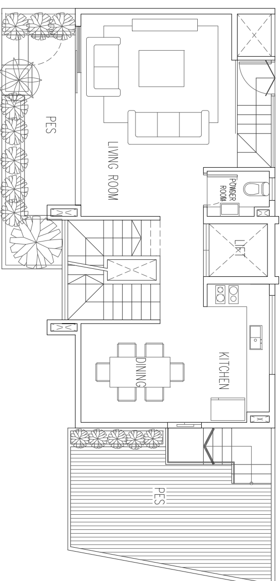
1ST STOREY
