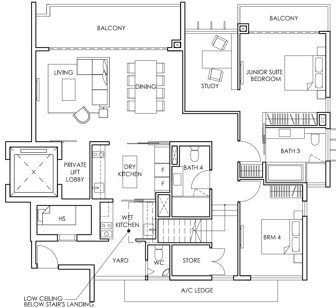
LOWER LEVEL
