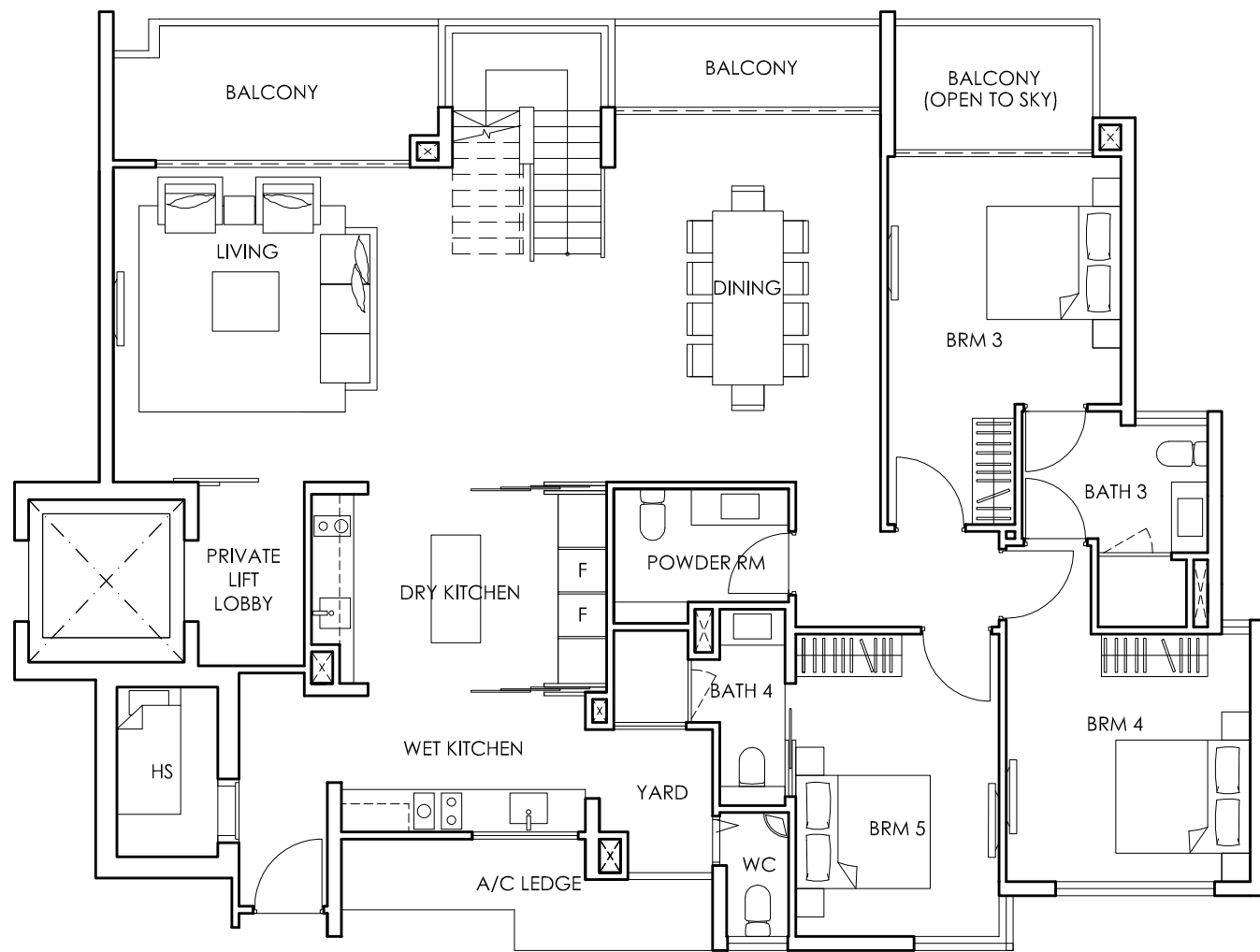
LOWER LEVEL
